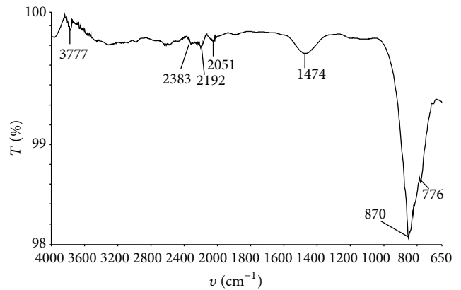
FIGURE 2: The FTIR spectrum of the LF slag.
