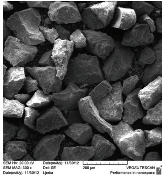
FIGURE 4: The SEM morphology of the LF slag particles.
