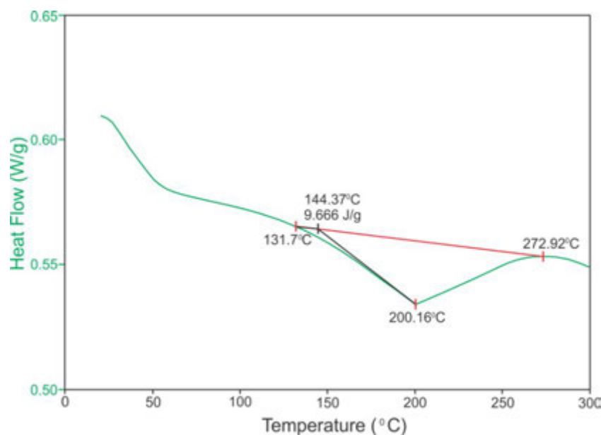
Figure 6. Part of the DSC heating curve for the sample 4 in the temperature range of the first detected endothermic peak related to martensite/austenite transformation
