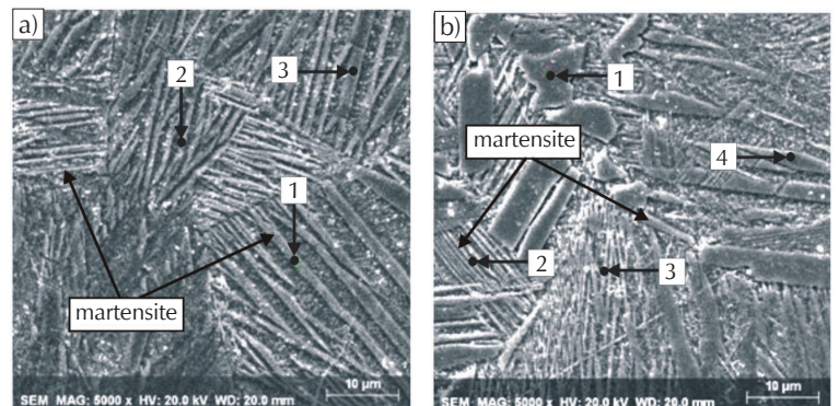
Fig. 4 – SEM micrographs of Cu-Al-Mn (a), and Cu-Al-Mn-Ti (b) shape memory ribbons after quenching with marked positions for EDS analysis
