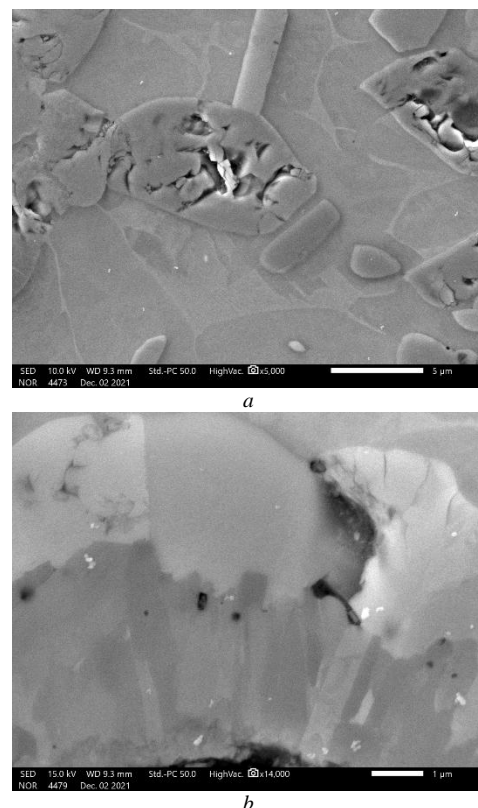
Fig. 4. Secondary electron scanning image of Ti-Al-C sample: a – porous carbides are visible inside \beta -Ti matrix; b – small cracks inside carbides (at the upper right corner of the image)
