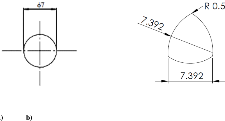
Fig. 3. Comparison of the ordinary and the new nails: a – comparison of the cross-section dimensions; b - view of the used nails with the new shape and \phi 7
