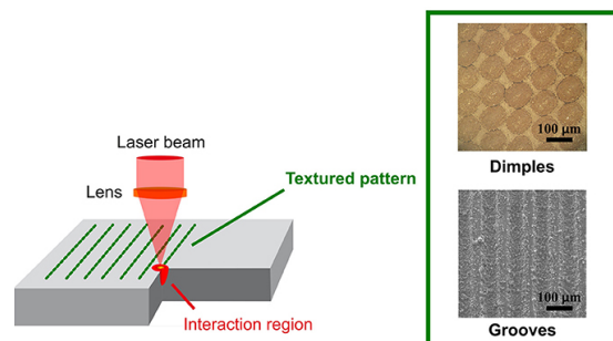
Fig. 2 The process of the surface texturing process with a laser beam [10]
