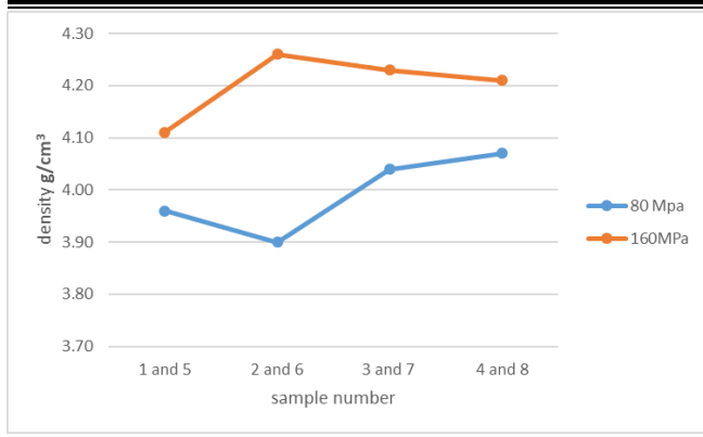
Fig. 1 Dependence of green density on applied pressing pressure.
