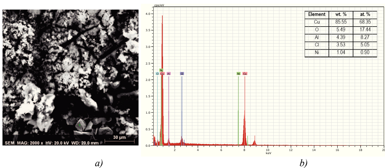
Figure 13. a) SEM images of the Cu-Al-Ni surface after potentiodynamic polarization measurement in 1.5% NaCl solution; b) EDS analysis
