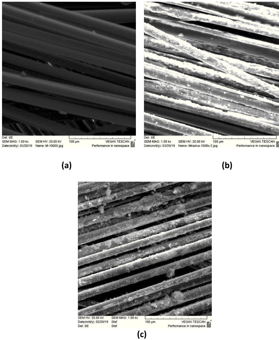
Figure 2. SEM images: (a) clean glass mesh, (b) glass mesh with TiO 2 , (c) glass mesh with TiO 2 / MWCNT
