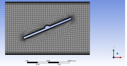
Fig. 10 Mesh for Throttle body B(75%)
