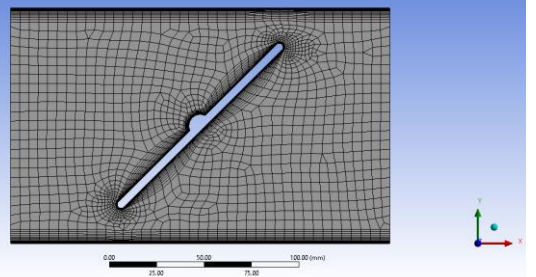
Fig. 11 Mesh for Throttle body B(50%)
