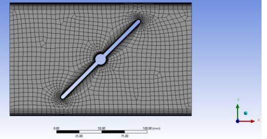
Fig. 8 Mesh for Throttle body A(50%)
