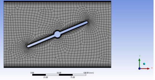
Fig. 7 Mesh for Throttle body A(75%)
