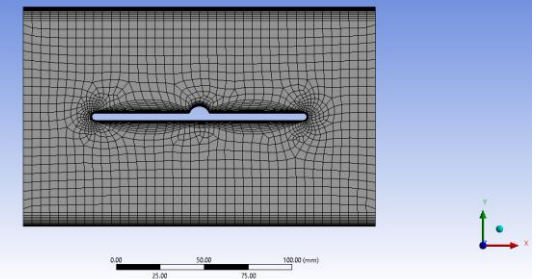
Fig. 9 Mesh for Throttle body B(100%)
