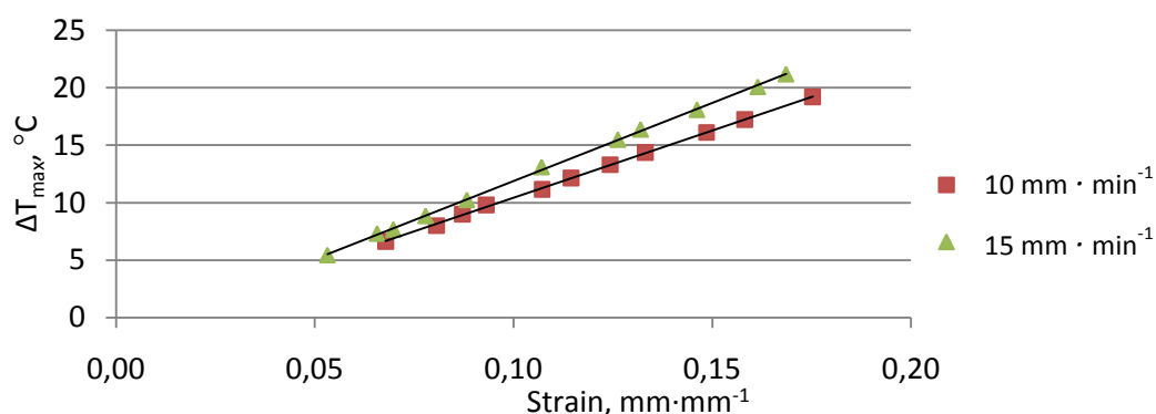
Figure 2. Dependence of temperature change on strain at different testing speeds
