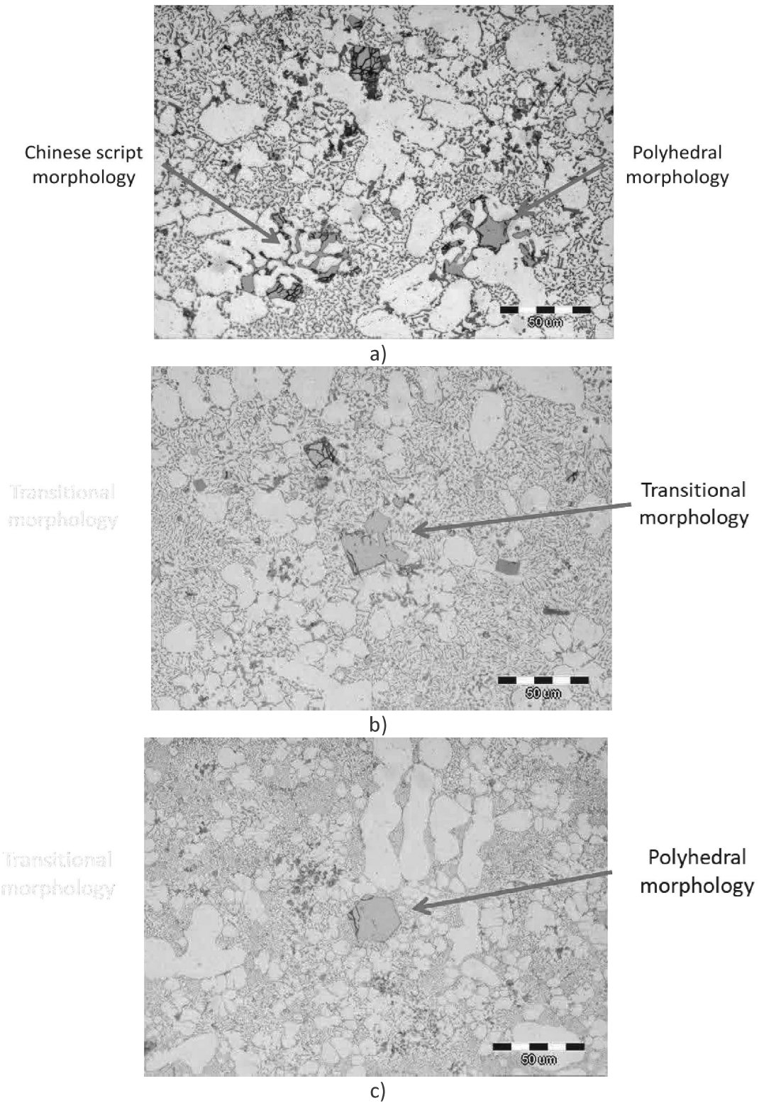
Figure 9. Microstructure of the samples showing: a) Chinese script morphology, b) Transitional morphology, c) Polyhedral morphology
