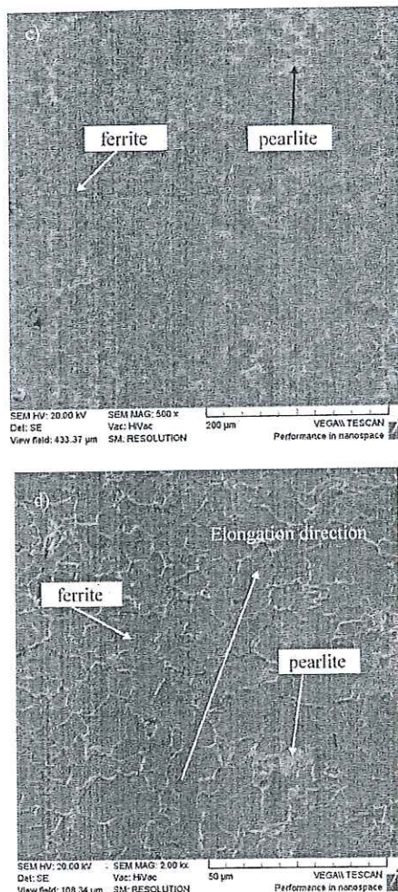
Fig.5. SEM micrographs of sample 2.
