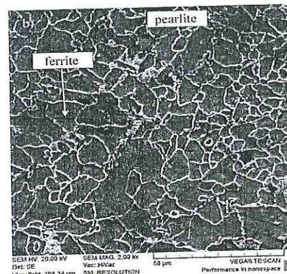
Fig.4. SEM micrographs of sample 1.
