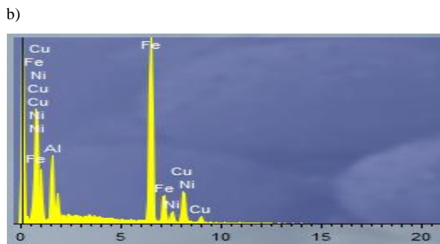
c) Fig. 5 Microstructure of quenched CuAl9Ni3Fe3 alloy after aging at 300 °C (a) results of EDS analysis of \alpha and \beta' phases (b) EDS analysis of one \kappa phase particle (c).
