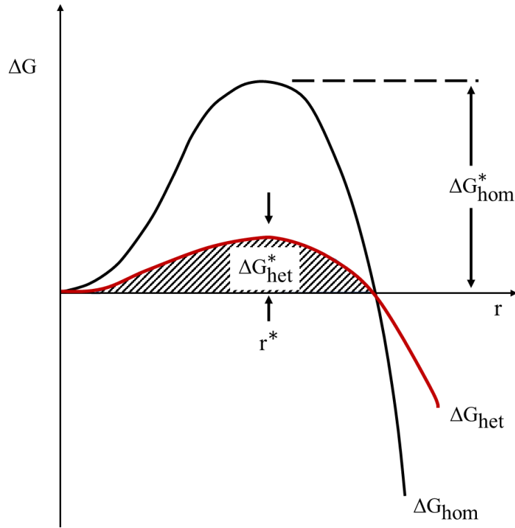
Figure 2.44. The excess free energy of solid clusters necessary for homogeneous and heterogeneous nucleation [334]
