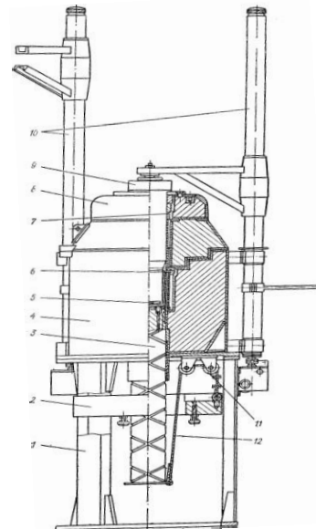
Fig. 2. Structural scheme of the "Issledovatel" gamma installation: 1 - bed; 2 - counterweight; 3 - stock; lead container (radiation head); 5 - work table; 6 - cylindrical irradiator; 7-beam shutter; 8-shutter body; 9-cork; 10-lift mechanism; 11 - blocks; 12-cables.
