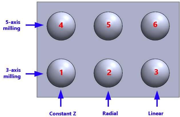
Fig. 2 The arrangement of the surfaces on the sample
