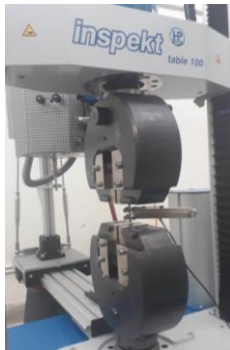
Fig. 3 Static tensile test conducted with extensometer
