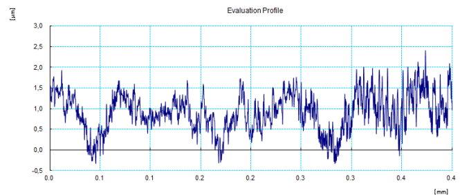
Fig. 9 Surface roughness measurement record
