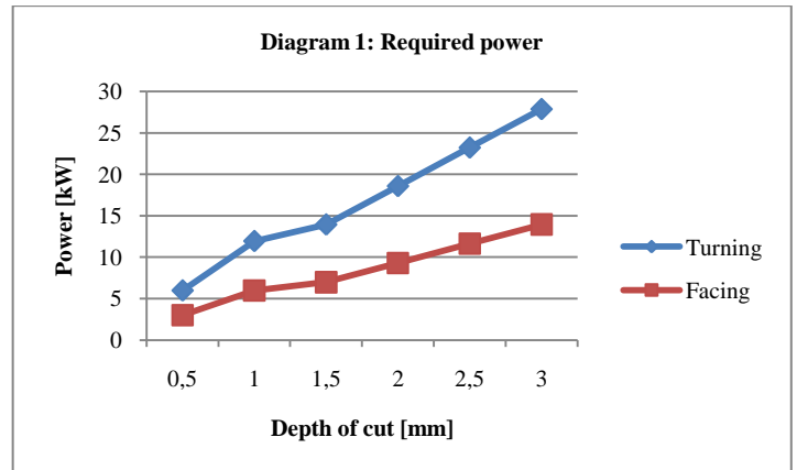
Fig. 3 Required power for turning and facing operations on the CNC Spinner EL-510 lathe
