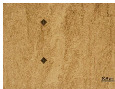
Fig. 7 Microstructure of fist cladded layer with Dievar
