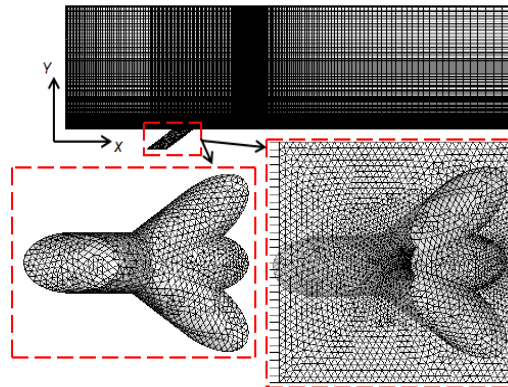
Figure 2. Meshes
