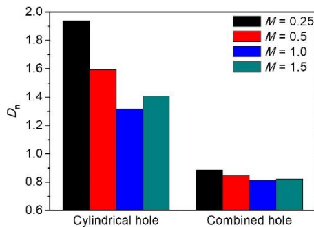
Figure 8. Non-uniformity distribution, D_n , for two-hole configurations at various blowing ratios
