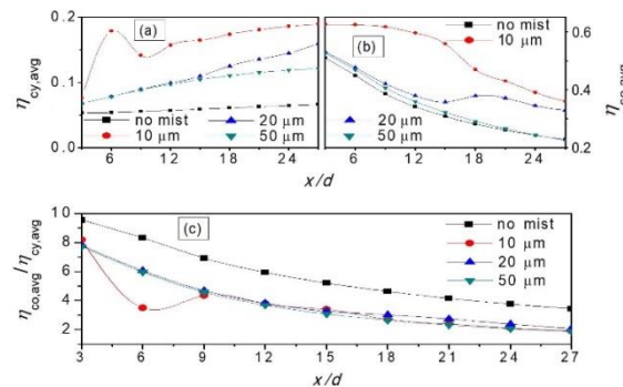
Figure 10. Lateral averaged film cooling effectiveness for the cases with different droplet sizes, M = 1.0
