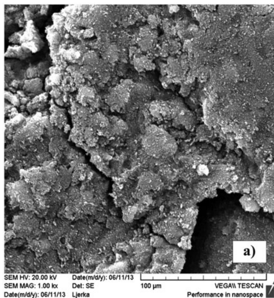
Fig. 2. SEM of the CB surface: (a) prior, and (b) following the Cr(VI) adsorption; c_i = 50 mg/L.
